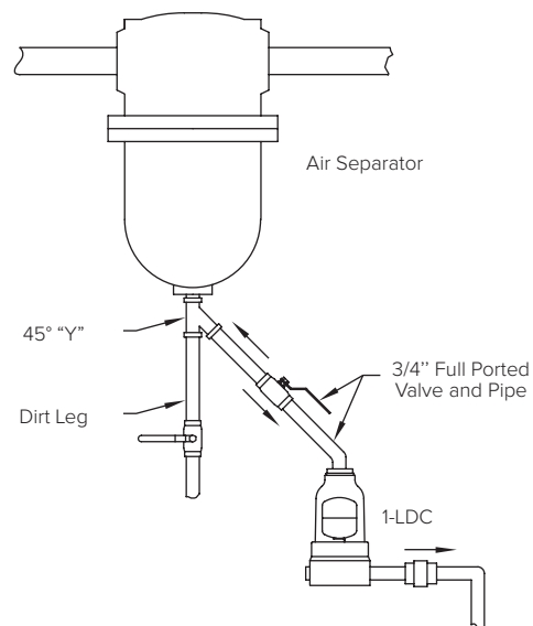
Figure LD-344-1. Typical Drain Trap Location
